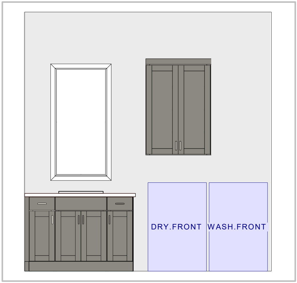
CABINETRY DRAWING
